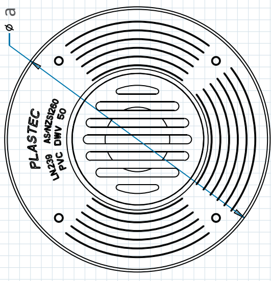
MEASUREMENTS (MM)
